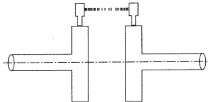
Laser Aligning
