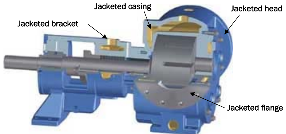
FULLY-JACKETED PUMP WITH JACKETED BRACKET, CASING, FLANGES & HEAD
